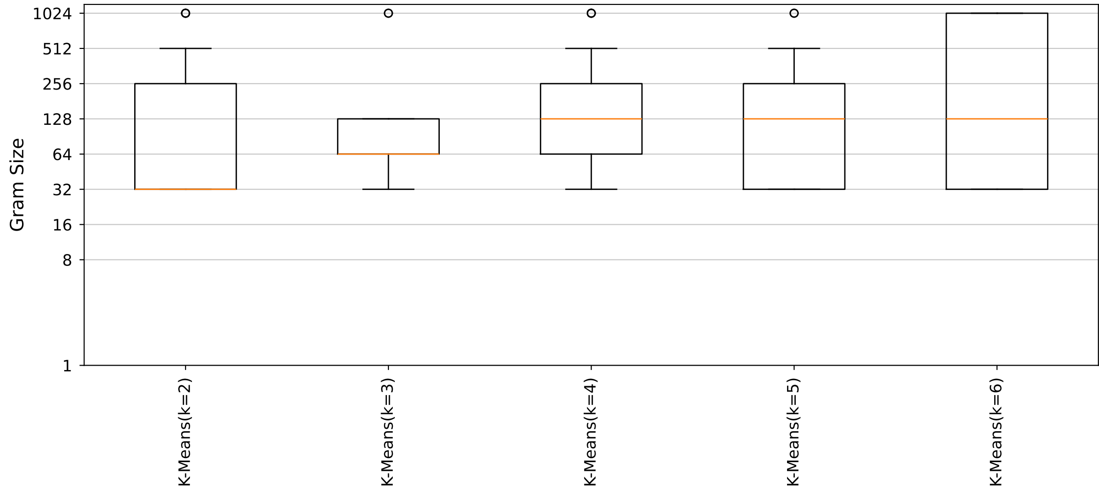
YARA Rules Gram Size Distribution (Cluster23_Size6 dataset)
